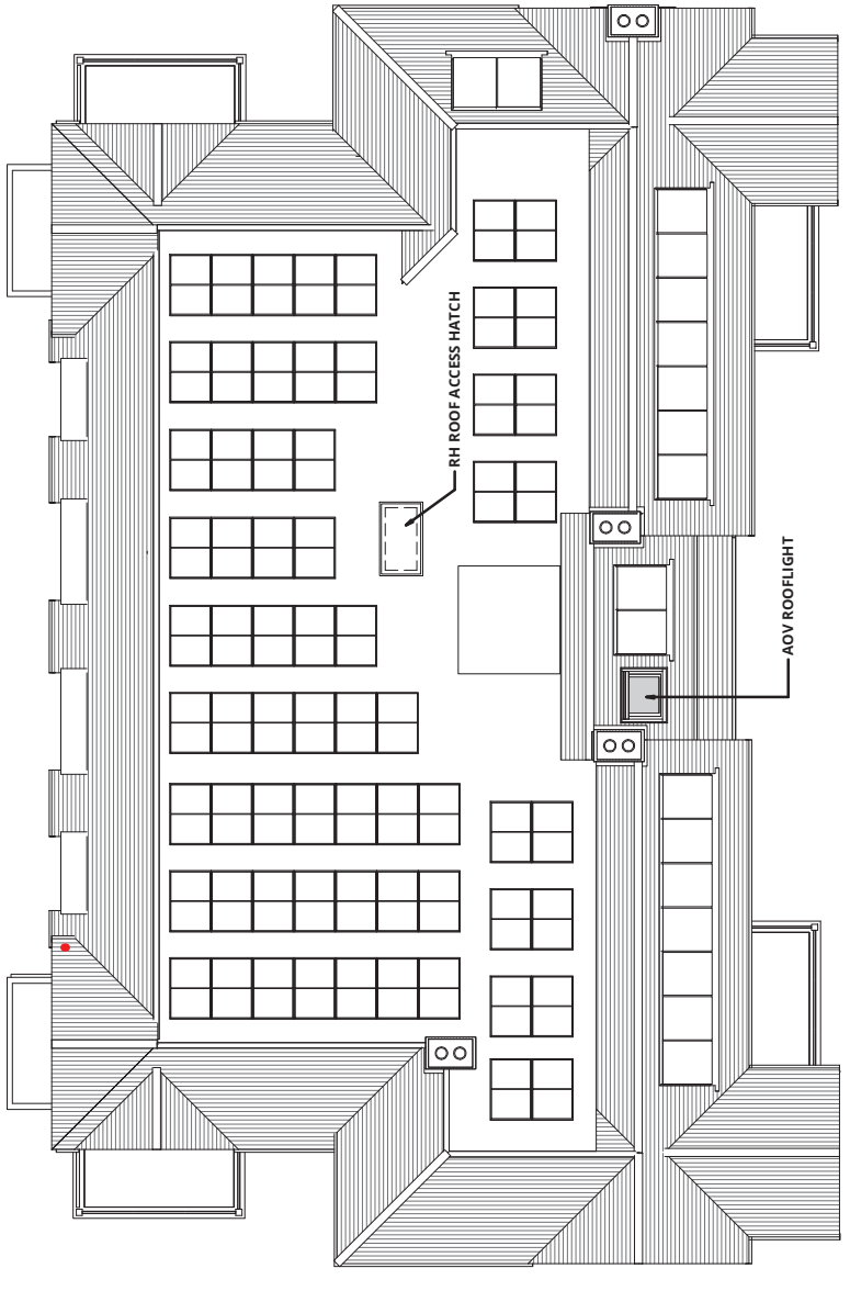
ROOF PLAN
